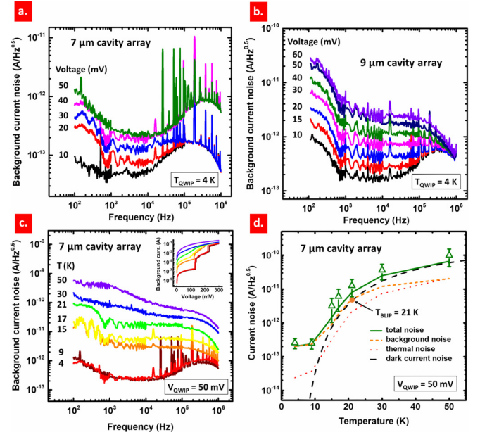
FIG. 2. Current noise spectral density measurements for THz QWIPs under background exposure. The background current noise for the (a) 7 \mu\text{m} and (b) 9 \mu\text{m} array devices at T = 4 \text{ K} is shown as a function of applied voltage, and (c) the background current noise for the 7 \mu\text{m} array device is shown as a function of temperature at V = 50 \text{ mV} . The Resistance amplifier is 10^6 and 10^7 \Omega for the 7 \mu\text{m} cavity array (a) and (c) and 10^6 \Omega for the 9 \mu\text{m} (b). The inset in (c) illustrates the dc current-voltage characteristics of the 7 \mu\text{m} array device, measured at the same temperature of the acquired noise spectra. (d) Comparison between measured current noise for the 7 \mu\text{m} cavity array QWIP at 10 \text{ kHz} and the estimated total background noise (continuous green line). The dashed orange and black lines show the background and dark current contributions, respectively. The dotted orange line represents the thermal noise contribution.
