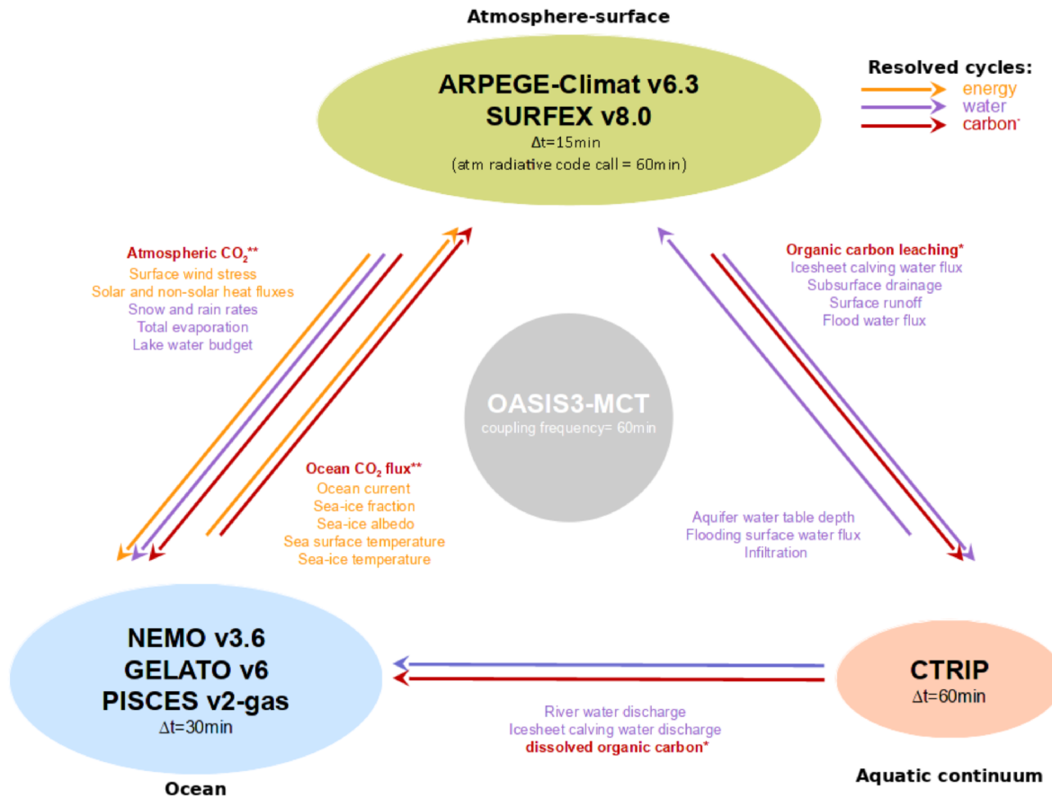
Figure 1. Overview of the coupling between CNRM-ESM2-1 components. t denotes model time step in minutes. Orange, blue, and red arrows give the direction of the exchange of energy, water, and biogeochemical fields between models. * denotes the biogeochemical fields that are used in all CNRM-ESM2-1 simulation, except in stand-alone configuration such as OMIP. ** denotes the biogeochemical fields that are used only in emission-driven simulations.
