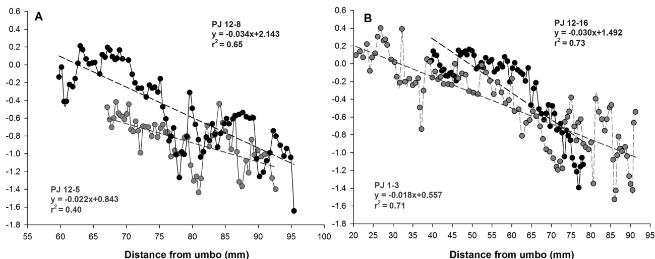
Fig. 4. Ontogenetic linear decrease in \delta^{13}\text{C}_{\text{shell calcite}} values versus shell height (distance from umbo) in Pecten jacobaeus A. specimens PJ 12-5 (dark grey) and PJ 12-8 (black), B. Specimens PJ 12-16 (black) and PJ 1-3 (dark grey). Linear regression lines, equations and determination coefficients shown in corresponding graphs.
