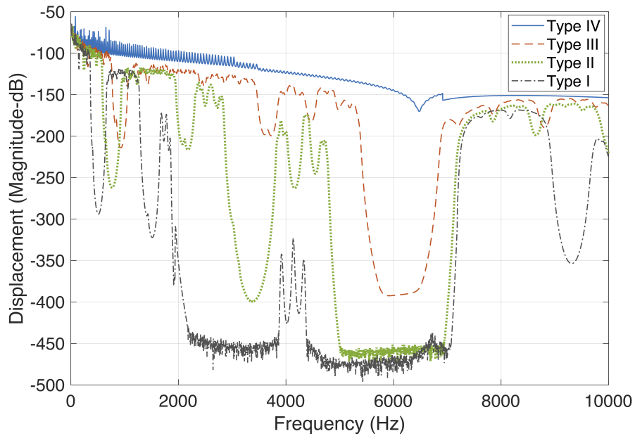
Figure 13: FRFs of the flexural waves for 11 th order of Fibonacci beam with geometrical variation
