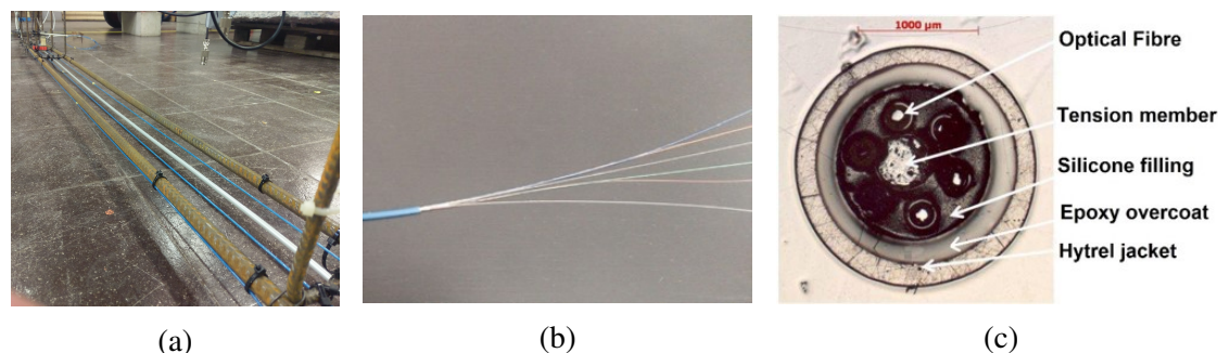
Figure 2: (a) Embedded optical fiber lines before concrete casting. (b) Photo of the optical cable [10]. (c) Micrography of different constitutive layers of the optical cable [11].
