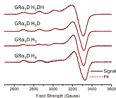
Figure 4. Electron Paramagnetic Resonance spectra of the constructs presented in this study recorded at pH 7.5. Fits were done using the program SpinCount.
