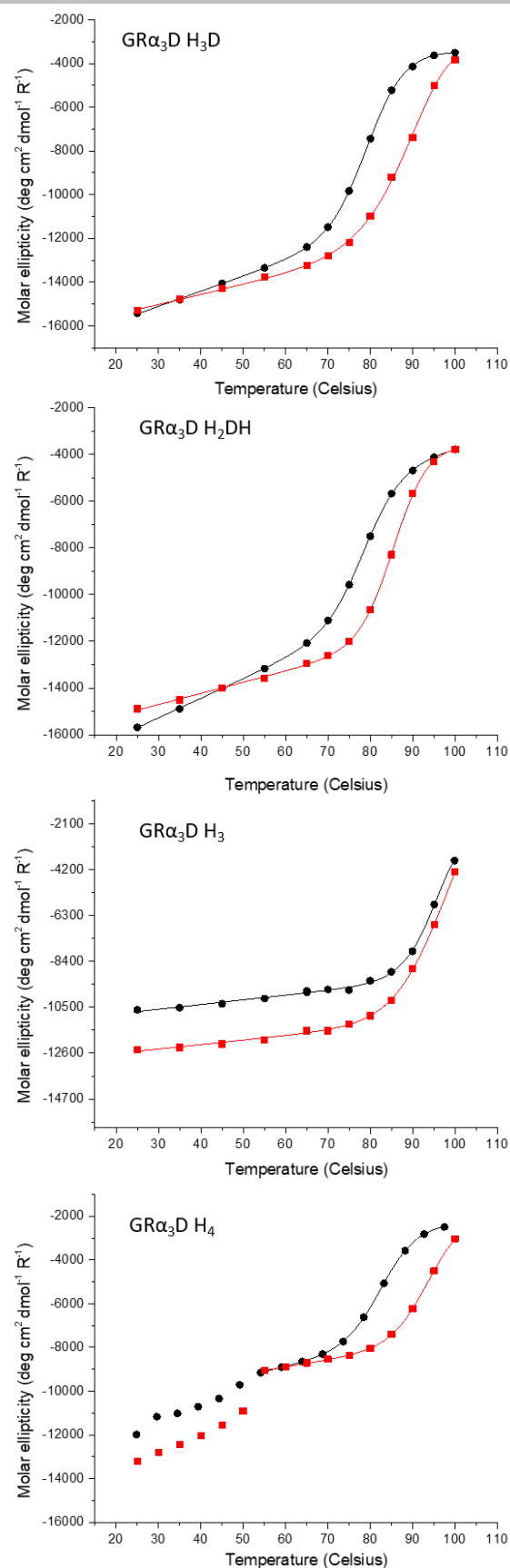
Figure 2. Thermal denaturation circular dichroism fits of GR \alpha_3 D H 3 D, H 2 DH, H 3 , and H 4 (top to bottom). Apo spectra are shown with black circles and Cu(II) bound spectra with red squares. Only the second denaturation step was fit for GR \alpha_3 D H 4 .
