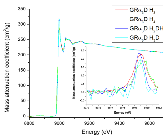
Figure 3. 1s → 3d region of Cu(II) XANES at pH 7.5 for every construct reported.
