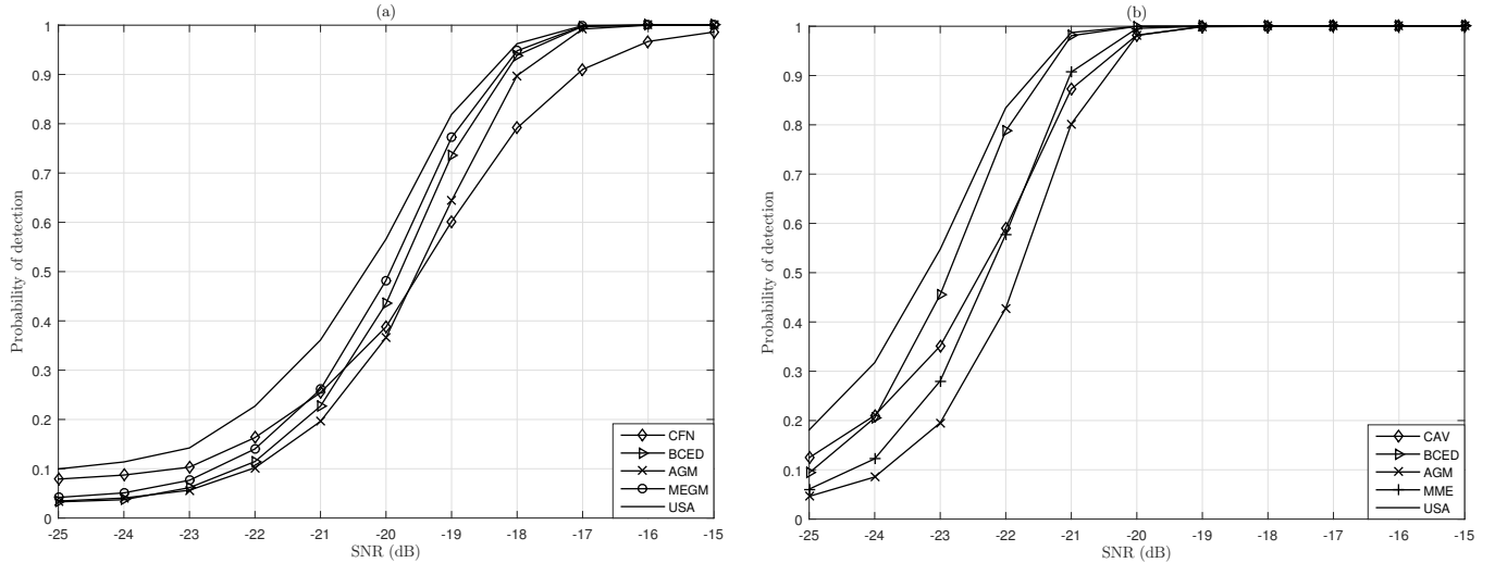
Fig. 4. Probability of detection versus SNR at different values of number of antenna M . (a) M = 4 and (b) M = 10 .
