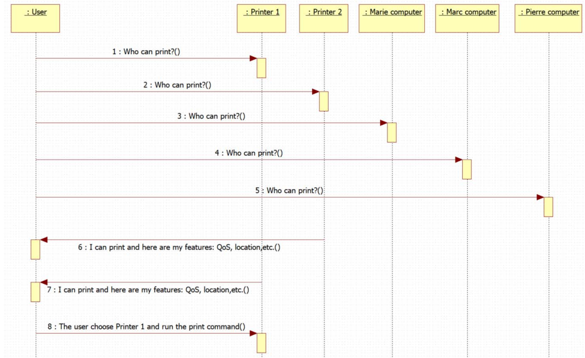
Figure 7: Sequence diagram
