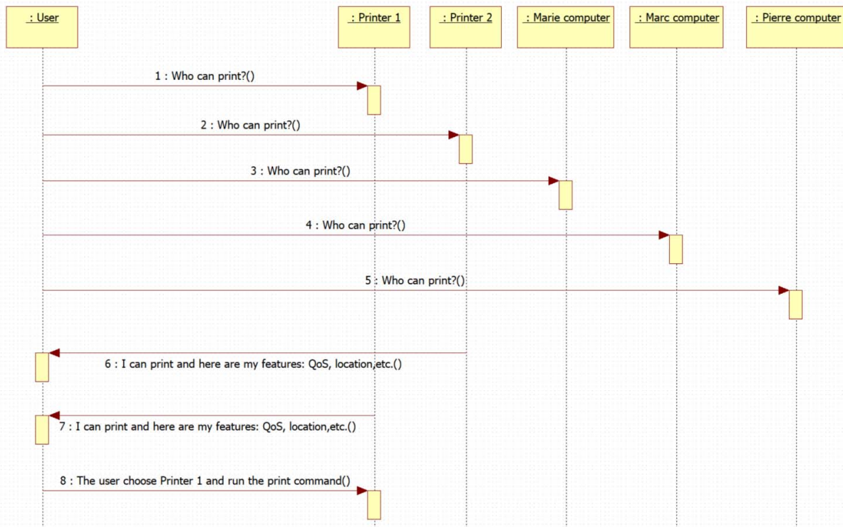
Figure 7: Sequence diagram
