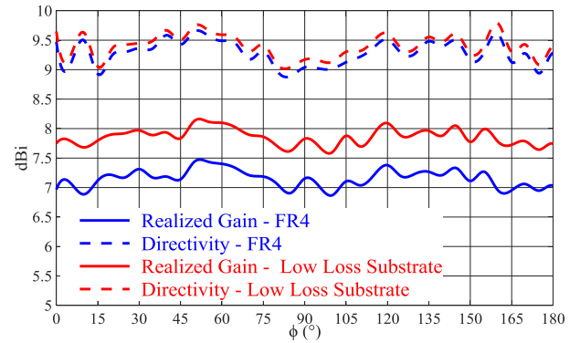
Fig.13. Comparison between a standard FR4 5x5 RPEA and a low loss substrate 5x5 RPEA toward the horizon ( \theta=90^\circ ) at frequency = 2.45 GHz
