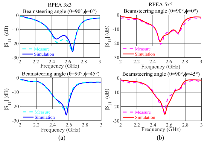
Fig. 10. Reflection coefficient on the fed part of the 3x3 RPEA (a) and the 5x5 RPEA (b) for two beamsteering angle \{\theta_0, \phi_0\} : \{90^\circ, 0^\circ\} and \{90^\circ, 45^\circ\}
