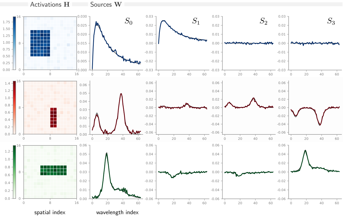
Fig. 1. QALS reconstruction example for the P = 3 sources case with \text{SNR}_{\text{dB}} = 0 dB. Reconstructed activations and Stokes parameters are given row-wise. Results display excellent match with theoretical values (solid black lines).
