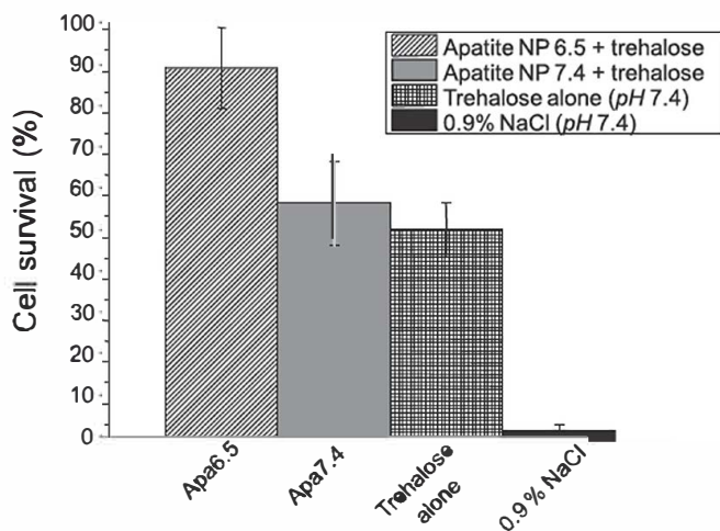
Fig. 5. RBC survival after freeze-thawing in different media (RBC were incubated in media for 7 h at 37 °C prior to freezing).
