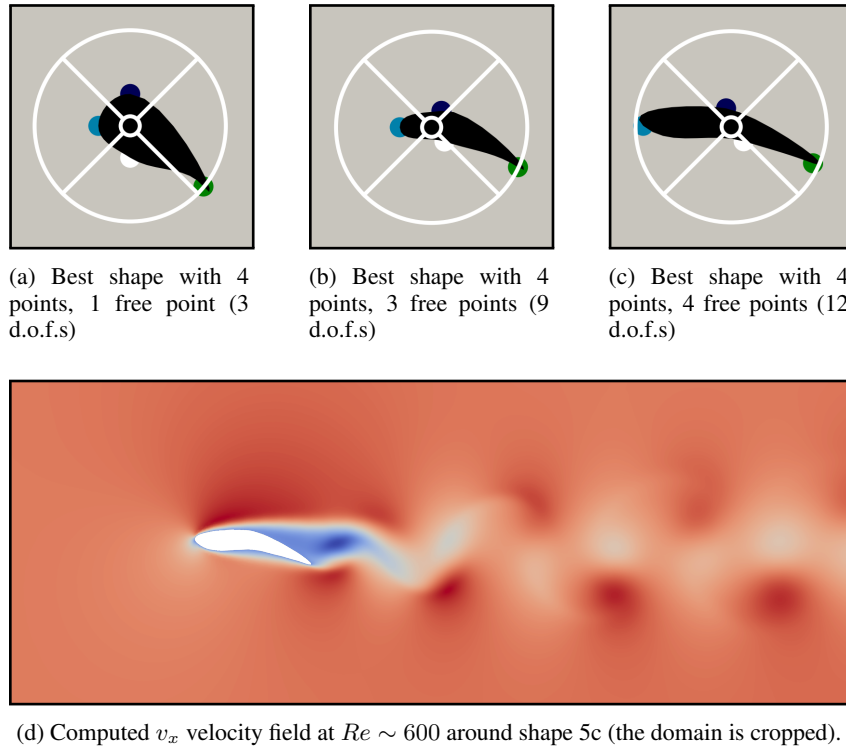
Figure 5: Results of the baseline shape optimization process. Best shapes obtained using 1, 3 and 4 free points are shown in subfigures 5a, 5b and 5c respectively. In subfigure 5a, the left, top and bottom points are fixed to their initial position ( i.e. that of the reference cylinder), while the rightmost one is free to move. In subfigure 5b, only the left point is fixed, while in subfigure 5c, all four points are free to move. The velocity field corresponding to shape 5c is shown in subfigure 5d.
