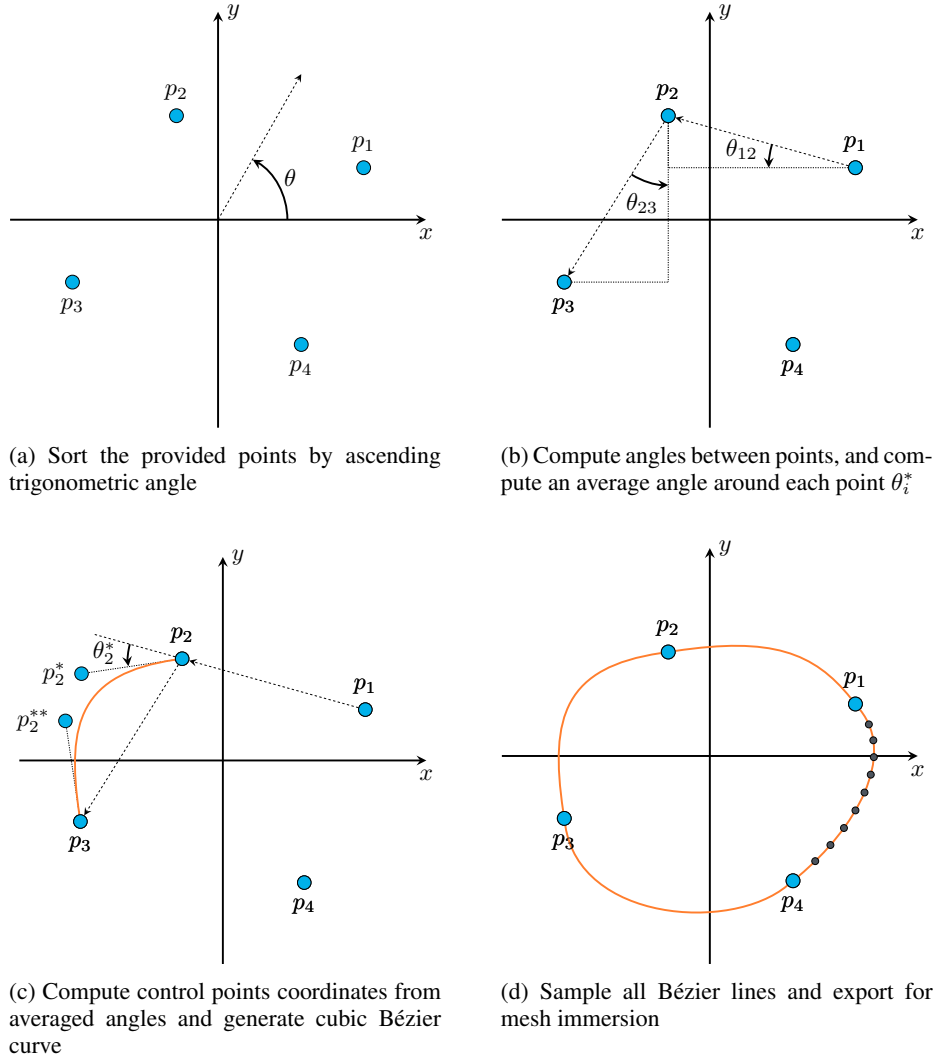
Figure 11: Shape generation using cubic Bézier curves. Each subfigure illustrates one of the consecutive steps used in the process. Detailed nomenclature is provided in the text.
