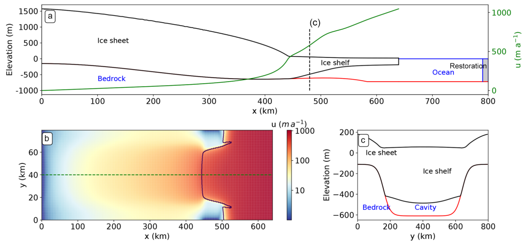
Figure 2. Initial ice-sheet in equilibrium calculated by Elmer/Ice with an accumulation rate of 0.3 \text{ m a}^{-1} and no sub-shelf melting as required by the MISMP+ protocol (Asay-Davis et al., 2016). (a) Side-view geometry in the central flow line, also indicating the position of the ocean restoration used by the ocean model, and the velocity magnitude along the central flow line shown in panel (b) . (b) Velocity magnitude seen from above. The black solid line indicates the grounding line. (c) Cross section of the ice sheet at x = 480 \text{ km} .
