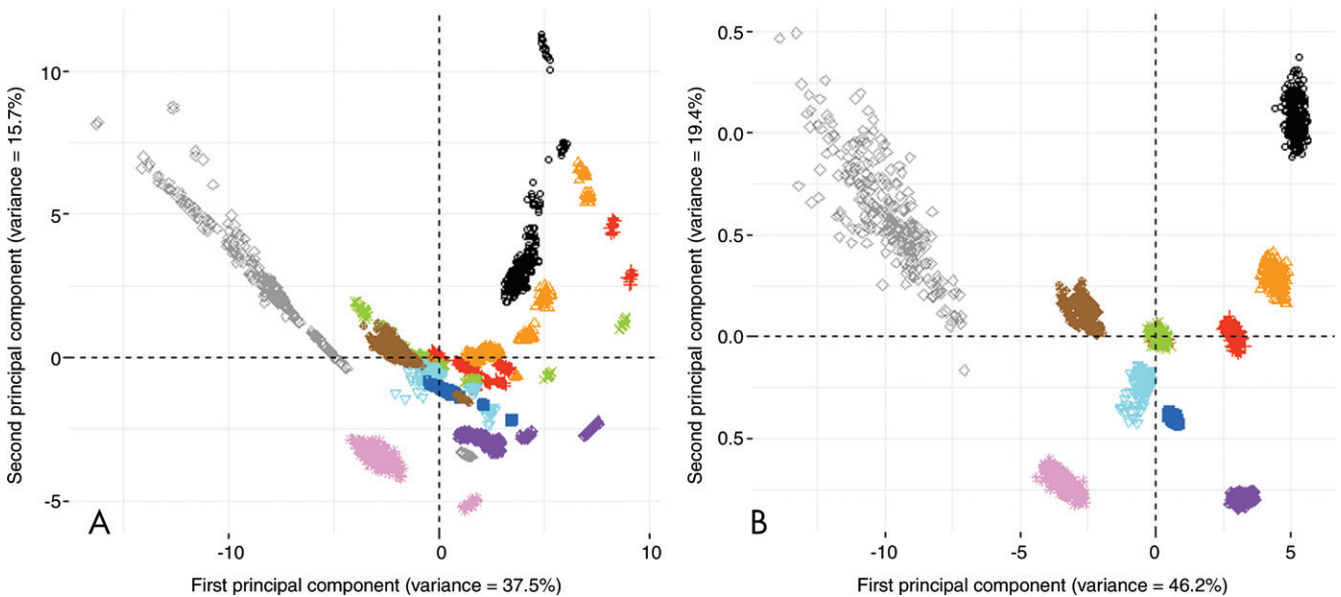
Figure 1: Phantom data: principal component scores for 2560 samples corresponding to 16 volume of interest × 10 texture patterns (represented by 10 different colors in the figure) × 16 imaging protocols described by 40 radiomic features on the first two principal components before, A, and after, B, ComBat ( https://github.com/Jfortin1/ComBatHarmonization ). After compensation, each texture pattern (ie, each color) was no longer composed of several separate and different clusters. Instead, the 10 texture patterns are nonoverlapping, demonstrating that the effect of the CT scanner protocol has been removed.
