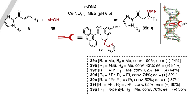
Figure 11. DNA-based asymmetric oxo-Michael addition.
