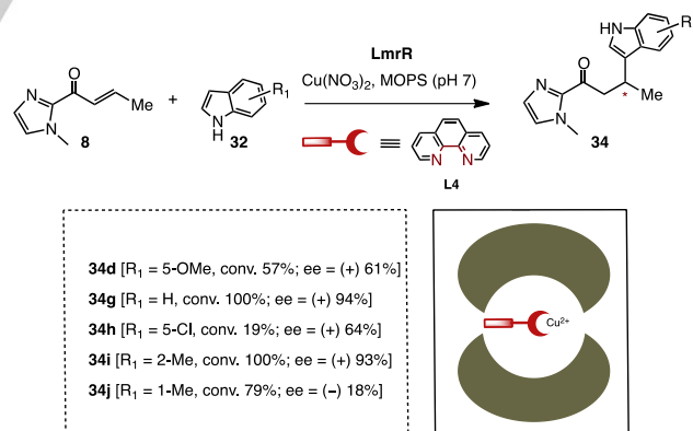
Figure 27. Supramolecular approach for the LmrR -based asymmetric Friedel-Crafts alkylation.
