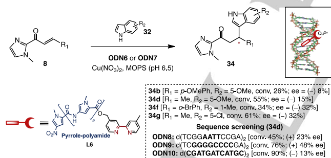
Figure 16. DNA-based asymmetric Friedel-Crafts alkylation using pyrrole-polyamide L6 .
