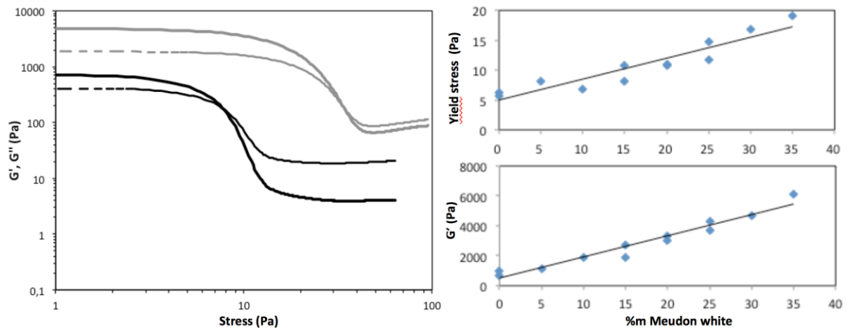
Figure 6: Rheological measurements on lead white based paints: left, viscoelastic properties of paints containing 0 wt% of chalk (black line) and 30 wt% of calcite (grey line). On the right, yield stress value and elastic modulus G' depending on the amount of chalk added to the lead white paint.
