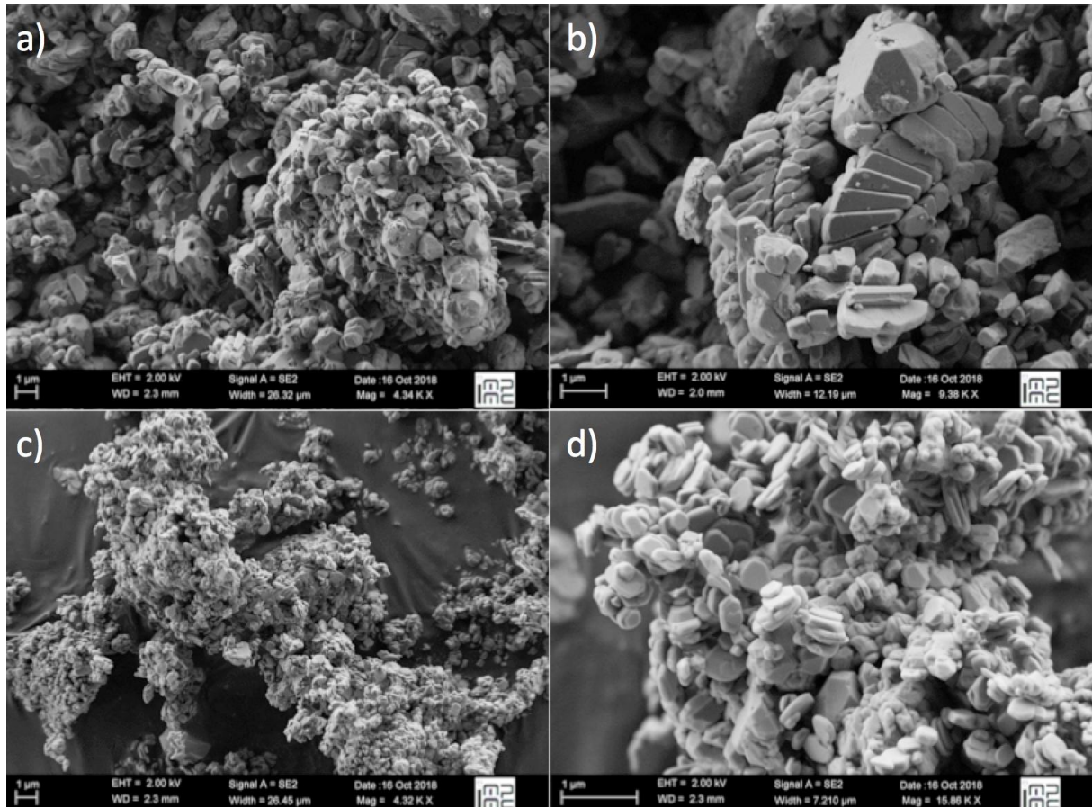
Figure 5: SEM images of a) and b) Meudon white from Laverdure and c) and d) lead white from Master's pigment.
