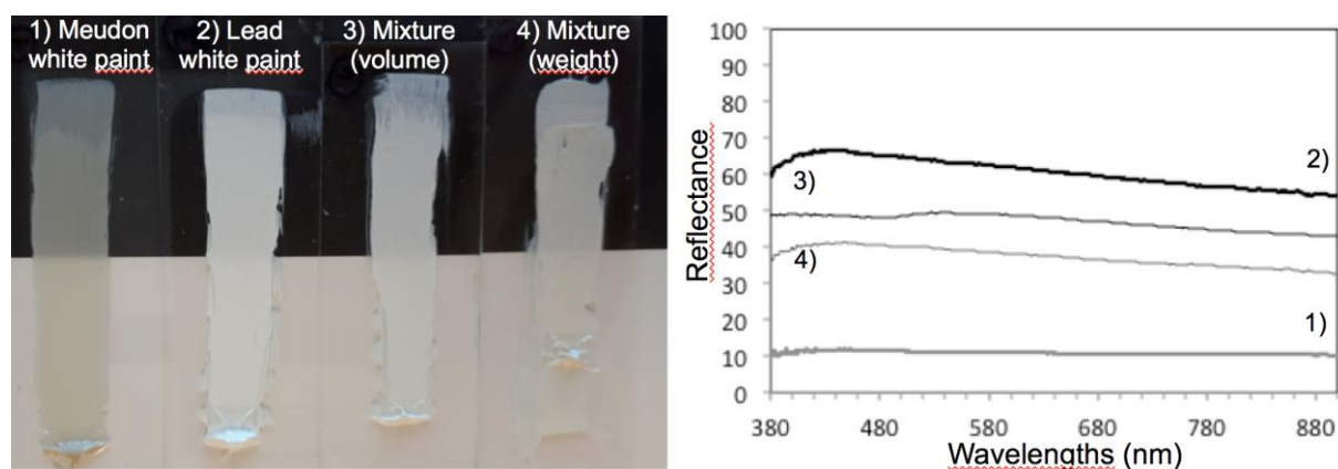
Figure 4: Photographs (left) and (right) visible reflectance spectra of the paint spread on a glass slide placed on the optical black (at t = 1 week) of: 1) Meudon white paint, 2) lead white paint and 3) and 4) the mixtures lead white (2 parts) + Meudon white (1 part) respectively in volume and in weight. The oil/pigment proportions used are detailed in the Experimental section.
