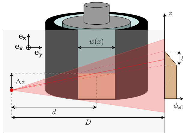
FIG. 12. Parallax issues along the vertical direction. For a pointlike source located at a vertical distance \Delta z from the suspension slab under study, volume fraction measurements are smoothed over a typical size \ell , proportional to the suspension thickness crossed by the X-rays w(x) and to \Delta z for small X-ray angles.
