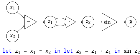
Fig. 1. A computational graph with inputs x_1 , x_2 and output y , and its corresponding term. Nodes are drawn as circles, hyperedges as triangles. The output y does not appear in the term: it corresponds to its root.
