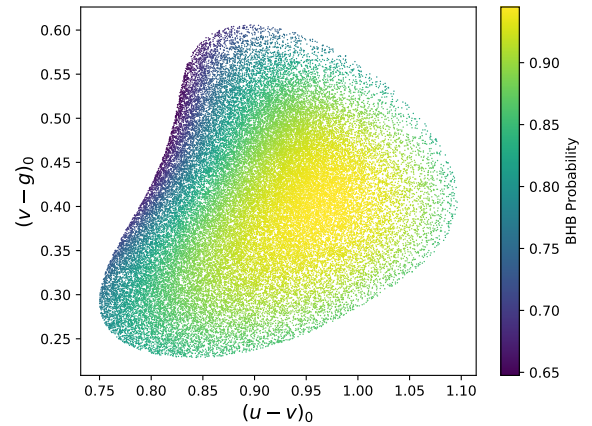
Figure 5. BHB stars from SkyMapper selected by our trained ANN. The probability of each stars being BHB star is presented by colour. Stars are concentrated at ((u-v)_0, (v-g)_0) , where the probability of being BHB stars is the highest.
