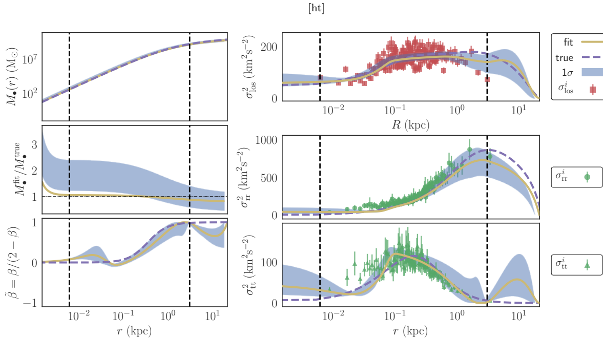
Figure 12. Same as Fig 8 for the NonPlumCoreOM 1k dataset. In the top right panel the \sigma_{\text{los}}^2 data are from the GAN synthetic data generator. In the two bottom right panels the \sigma_{\text{rr}}^2 and \sigma_{\text{tt}}^2 moments are from the true NonPlumCoreOM 10k dataset (we do not have 3D motions for the GAN generated data).
