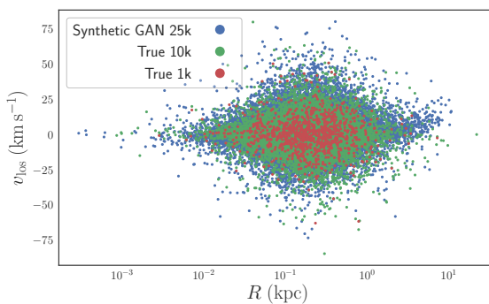
Figure 3. Comparison of NonPlumCoreOM 1k, 10k true datasets against the GAN generated synthetic data on the (R, v_{\text{los}}) plane.
