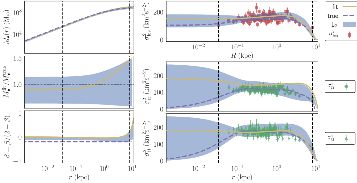
Figure 10. Same as Fig 8 for the PlumCuspTan 10k dataset.
