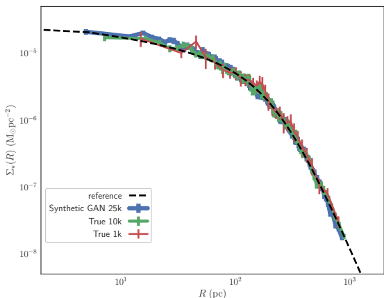
Figure 5. Comparison of NonPlumCoreOM 1k, 10k true projected density profiles against the GAN generated projected density profile. Overplotted is the true reference profile.
