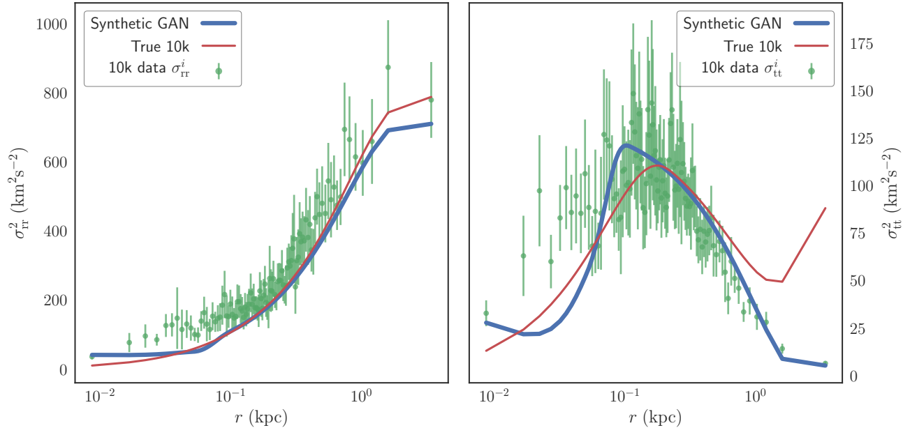
Figure 13. Difference in fitted profiles in latent profiles \sigma_{rr}^2 , \sigma_{tt}^2 for the models trained on the GAN generated synthetic dataset and the 10k dataset, for the NonPlumCoreOM model.
