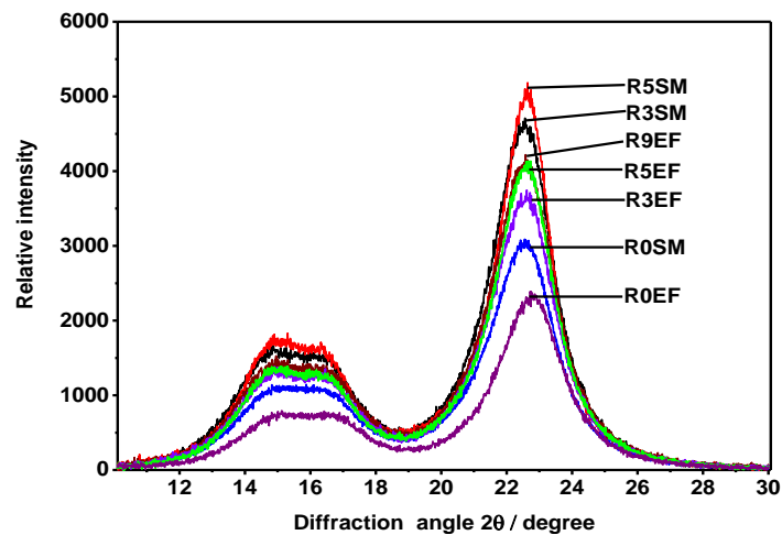
Figure 7. X-ray diffractograms of the fibres collected at different retting duration for EF and SM periods.
