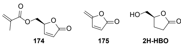
Chart 16. Methacrylated HBO , 174 , 5-methylene-2(5 H )-furanone, 175 and 2H-HBO .
