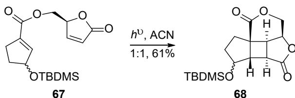
Scheme 14. First internal [2+2] photocycloaddition of a HBO derivative.
