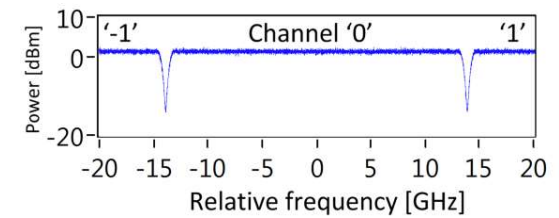
Fig. 13 The reduced phase noise MLL is modulated with data in 16-QAM format. Nyquist pulse shaping is used to obtain flat spectrum after data modulation. (a) shows the entire spectrum of the modulated MLL (b) zooms in on a portion to show the spectral guardband between the channels.
