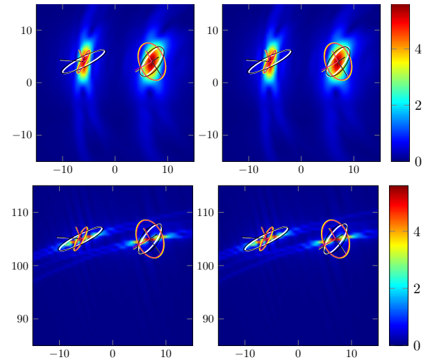
Figure 1: Cross-range (top) and range (bottom) images of \|\tilde{\alpha}(\cdot)\|_F . The columns show reconstructions with \Pi (left) and with p(\psi) (right). Here (up to a reference phase [1]) the true tensor \text{Re } \tilde{\alpha} (resp. \text{Im } \tilde{\alpha} ) is depicted by the white (resp. yellow) ellipses/axes, whereas the recovered tensor is depicted using black (real part) and magenta (imaginary part) ellipses/axes.
