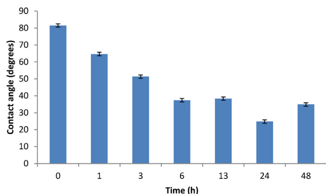
Fig. 2. Water contact angle of etched Ti6Al4V using 30 wt% H 2 O 2 aqueous solution for 0, 1, 3, 6, 13, 24 and 48 h; error bars correspond to standard deviation, with number of samples n = 3.
