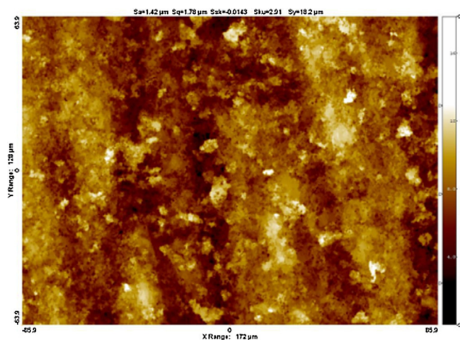
Fig. 5. White light interferometry of the surface of a hydroxyapatite tablet prior to coating with peptides. The average roughness was S_a = 1.42 \mu\text{m} .
