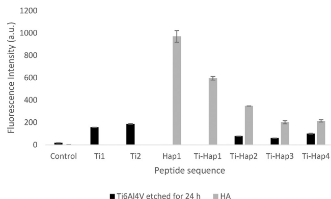
Fig. 4. Fluorescence Intensity on Ti6Al4V surfaces etched for 24 h and HA surfaces. Samples were immersed in a 1 \mu M concentration of peptide in PBS for 17 h; The error bars correspond to standard deviation, with number of samples n = 3. Control surfaces were uncoated; the Ti-Hap1 coating on the Ti6Al4V surface was visibly heterogeneous, and therefore the fluorescence intensity was not calculated. The set-up of the fluorescence microscope varied between the Ti6Al4V and HA surface measurements, and therefore intensity comparisons are not possible between the two different materials.
