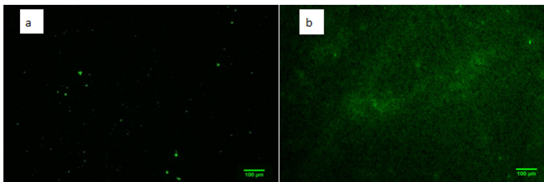
Fig. 3. Fluorescence microscopy images with 10X magnification (100 \mu m scale bar) of Ti6Al4V samples coated with Ti1 peptide, using a 1 \mu M concentration in PBS solution. Prior to coating, samples were polished to mirror finish and then etched using 30 wt% H 2 O 2 aqueous solution for (a) 1 h and (b) 24 h.
