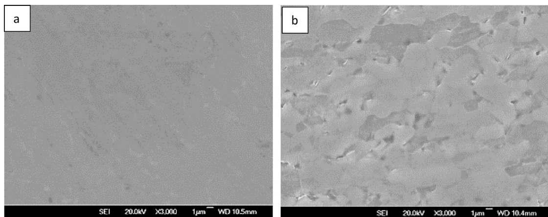
Fig. 1. SEM micrographs X3000 of (a) polished to mirror finish Ti6Al4V surface; (b) polished to mirror finish Ti6Al4V surface after etching for 24 h.
