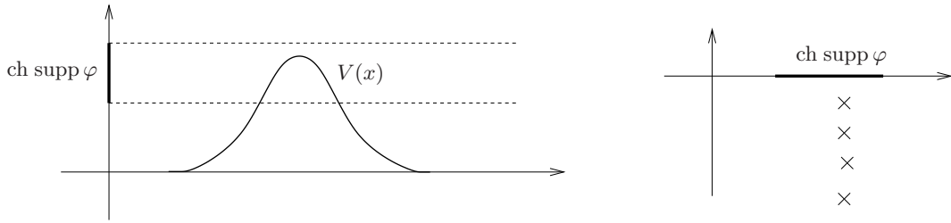
FIGURE 5. The geometric setting and the resonances of Q in Example 3.9.
