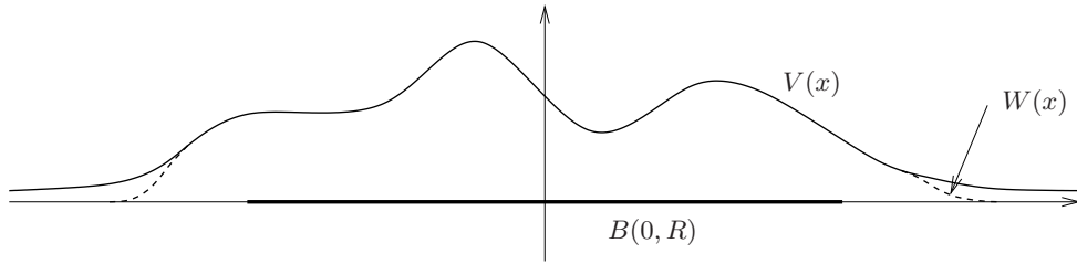
FIGURE 1. The potentials V and W given by (A2).
