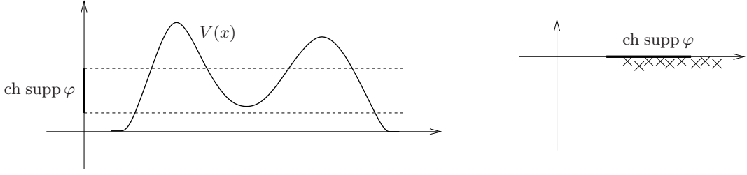
FIGURE 4. The geometric setting and the resonances of Q in Example 3.7.
