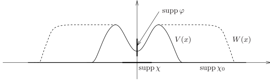
FIGURE 3. The setting in the proof of Remark 3.4.
