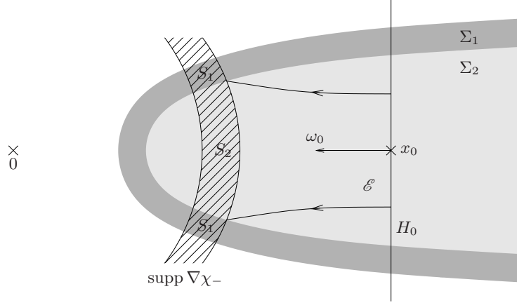
FIGURE 12. The geometric setting in the proof of Theorem 5.6.
