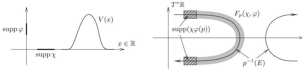
FIGURE 2. On the left, an example of potential V in dimension n = 1 . On the right, the associated set F_p(\chi, \varphi) and the energy surface p^{-1}(E) for some E \in \text{supp } \varphi .
