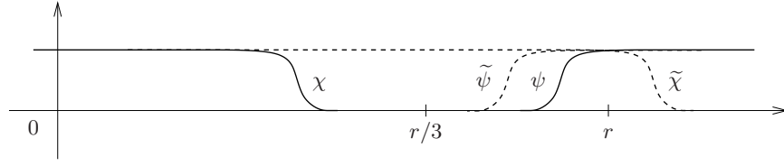
FIGURE 13. The various functions in the proof of Theorem 2.1.
