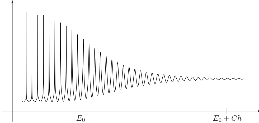
FIGURE 7. The derivative of the SSF given by Corollary 4.7.
