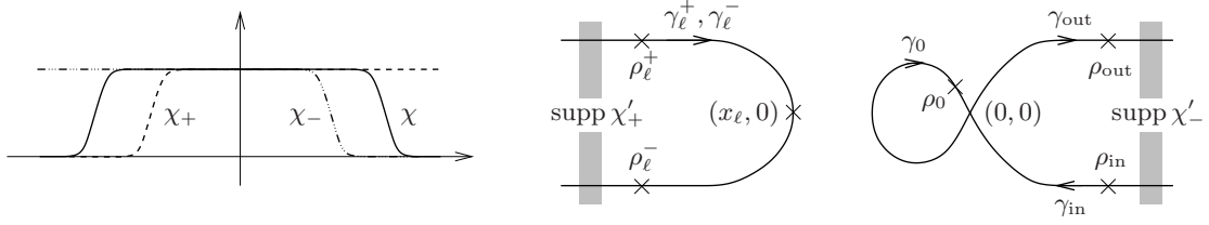
FIGURE 8. The cut-off functions \chi_\star and the geometry of Corollary 4.7.
