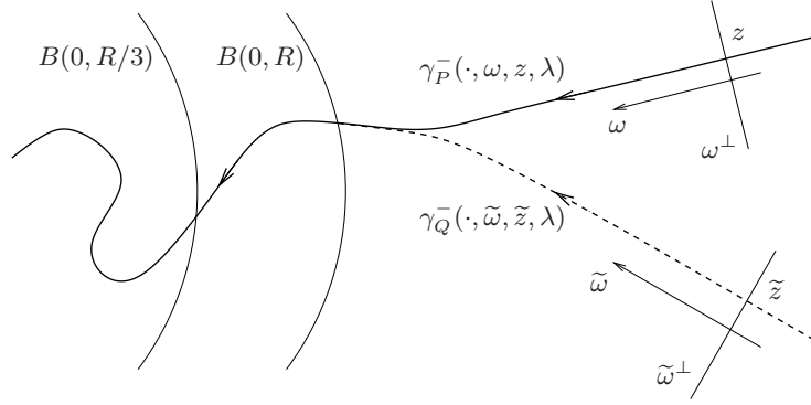
FIGURE 11. The canonical relation \Lambda_{Q \leftarrow P}^{\text{ini}} .
