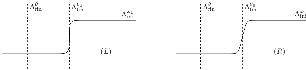
FIGURE 10. A cross section of the Lagrangian manifolds \Lambda_\bullet^* .
