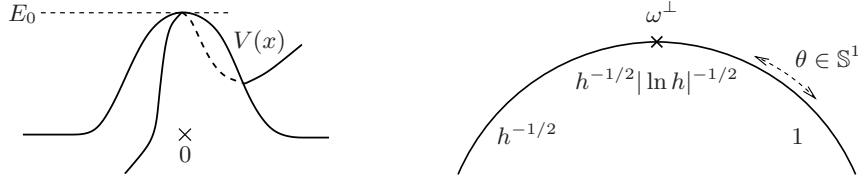
FIGURE 9. The potential of Example 5.1 and the order of the scattering amplitude in function of the final direction \theta \in \mathbb{S}^1 .
