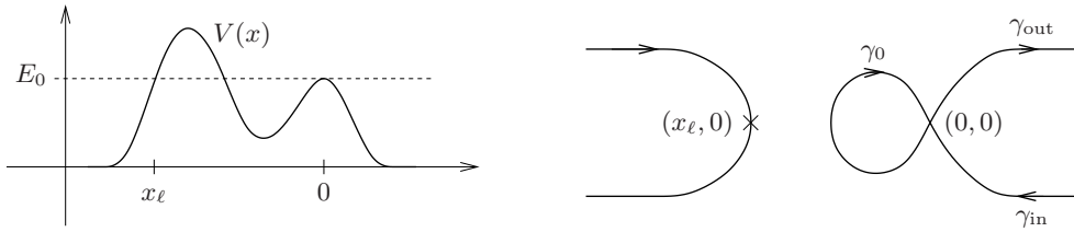
FIGURE 6. The geometric setting of Example 4.6.
