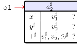
Figure 8. Join of all the results at the end of the loop body in Figure 7
