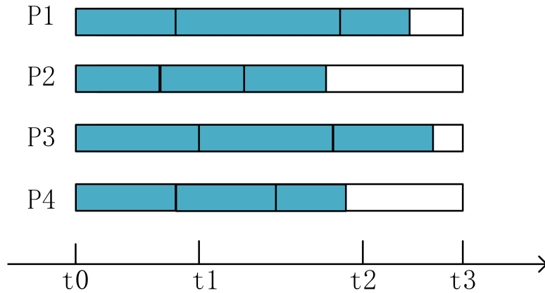
Figure 2: Asynchronous iterations
