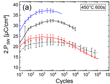
Fig. 8: For the case of 450°C 600s anneal, (a) mean 2.P_{SW} of 10 capacitors ( \varnothing 100\mu\text{m} ) along cycling for four different pulse conditions ( t_r & t_f = 100ns) and (b) 2.P_{SW}^{Max} achieved during square pulse cycling as a function of the corresponding die's CBD, illustrating the trade-off between switched polarization values and maximum endurance reached upon programming conditions.
