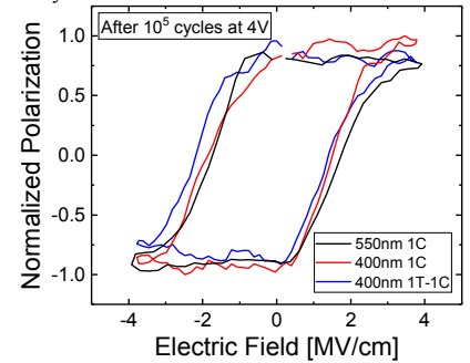
Fig. 18: Normalized polarization measured on BEOL integrated single 1C ( \text{\O}550\text{nm} ) and 1T-1C ( \text{\O}400\text{nm} ) through an open transistor ( V_G=5\text{V} ).
