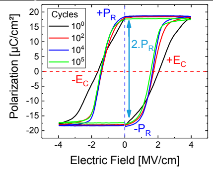
Fig. 3: PUND-corrected P-E measured at 10kHz +/-4V on \text{\O}100\mu\text{m} TiN/HZO/TiN capacitor annealed at 450°C 600s, to derive accurately 2.P_R values. Cycling has been performed with a 100kHz +/-4V triangular signal.
