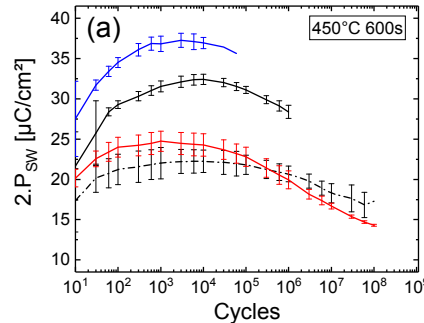
Fig. 8: For the case of 450°C 600s anneal, (a) mean 2.P_{SW} of 10 capacitors ( \text{\O}100\mu\text{m} ) along cycling for four different pulse conditions (tr & tf = 100ns) and (b) 2.P_{SW}^{Max} achieved during square pulse cycling as a function of the corresponding die's CBD, illustrating the trade-off between switched polarization values and maximum endurance reached upon programming conditions.
