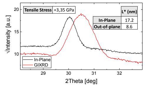
Fig. 15: From the GIXRD and the in-plane XRD patterns, the crystallite sizes ( L^* ) and the layer stress are extracted from the 0111 peak widths and positions, respectively.
