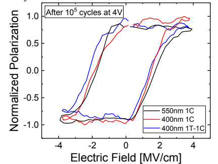
Fig. 18: Normalized polarization measured on BEOL integrated single 1C ( \text{\O}550\text{nm} and \text{\O}400\text{nm} ) and 1T-1C ( \text{\O}400\text{nm} ) through an open transistor ( V_G=5\text{V} ).
