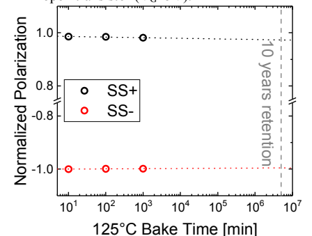
Fig. 21: Same State (SS) with positive (SS+) and negative (SS-) programming condition (see [10]) data retention at 125^\circ\text{C} measured on bitcells routed in parallel.
