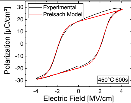
Fig. 2: Raw P-E plot on \text{\O}100\mu\text{m} TiN/HZO/TiN capacitor annealed at 450°C 600s and corresponding simulated curve derived from the Preisach-based model for accurate circuit simulations.
