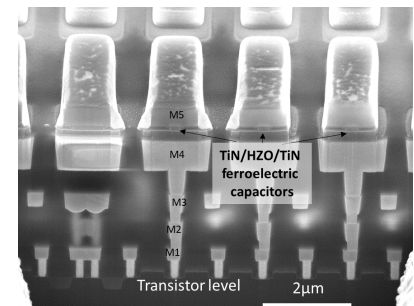
Fig. 12: SEM cross section showing the transistor level, the different metal lines, and \text{\O}300\text{nm} ferroelectric capacitors TiN/HZO/TiN integrated between M4 and M5.
