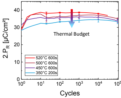
Fig. 4: 2.P_R values (mean and stand. dev.) reported along triangular cycling (4V/100kHz) for 10 TiN/HZO/TiN capacitors ( \text{\O}100\mu\text{m} ) after various anneals. HZO is demonstrated to be ferroelectric down to BEOL compatible thermal budgets with a minor decrease of 2.P_R .
