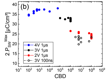
Fig. 8: For the case of 450°C 600s anneal, (a) mean 2.P_{SW} of 10 capacitors ( \text{\O}100\mu\text{m} ) along cycling for four different pulse conditions (tr & tf = 100ns) and (b) 2.P_{SW}^{Max} achieved during square pulse cycling as a function of the corresponding die's CBD, illustrating the trade-off between switched polarization values and maximum endurance reached upon programming conditions.
