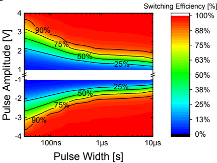
Fig. 7: Switching efficiency map for different square pulse widths (rise time (tr) & fall time (tf) = 100ns) and amplitudes, with a PUND 2.P_R as reference, on a \text{\O}100\mu\text{m} 450°C 600s annealed TiN/HZO/TiN capacitor, revealing programming conditions compatible with memory operations.
