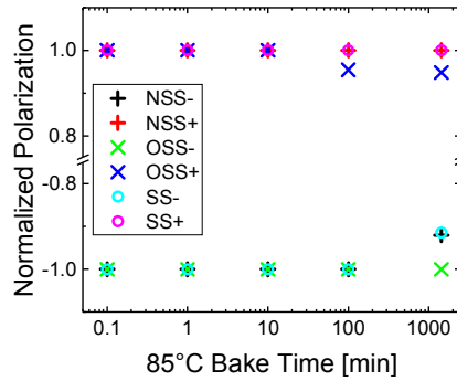
Fig. 5: Data retention up to 1440min baking time at 85°C on \text{\O}100\mu\text{m} capacitors measured with state-of-the-art FeRAM reliability characterizations [10].
