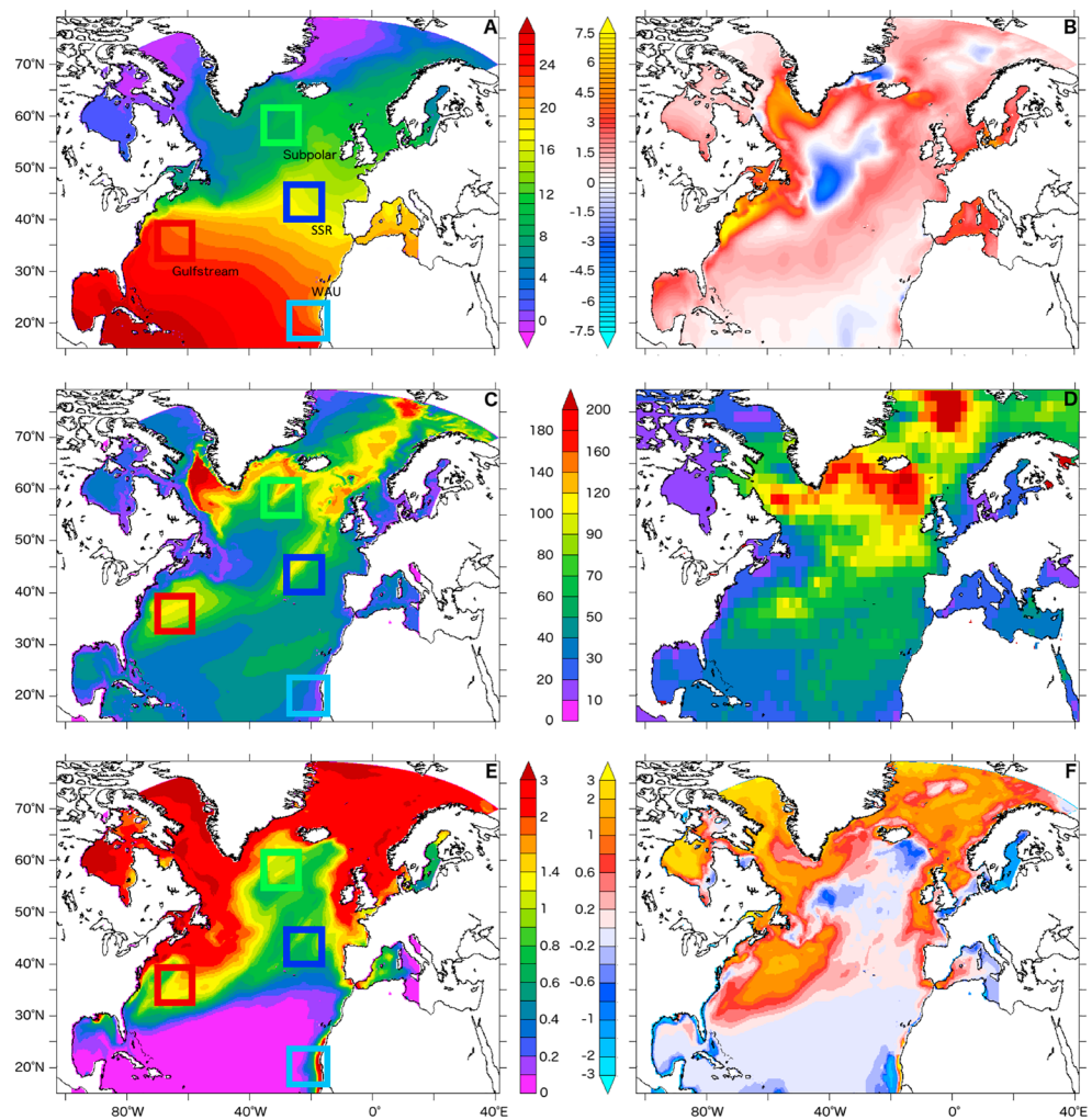
Figure 1. (a) Model Sea Surface Temperature (SST, °C) averaged between 2000 and 2005. Regions of interest are indicated: Subpolar (in green box), Subtropical Seasonally Stratified (SSR, in blue box), West African Upwelling (WAU, in light blue box), and Gulf Stream (in red box). (b) Difference between the simulated SST and the World Ocean Atlas (WOA) SST (Locarnini et al., 2006). (c) Annually averaged simulated mixed layer depth (m) over 2000 to 2005. (d) Observed Mixed layer depth (m) climatology from de Boyer Montégut et al. (2004). (e) Monthly climatological maximum surface Chlorophyll- a ( \text{mgC}/\text{m}^3 ) over the 2000 and 2005 period in CTL. (f) Difference ( \text{mgC}/\text{m}^3 ) between the monthly climatological simulated maximum of surface Chlorophyll and a climatology of the monthly maximum from the SeaWiFS Chlorophyll- a .
