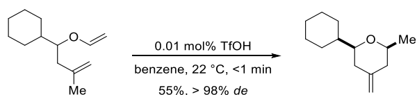
Scheme 11. Catalytic Prins -cyclisation of an unsubstituted enol ether.
