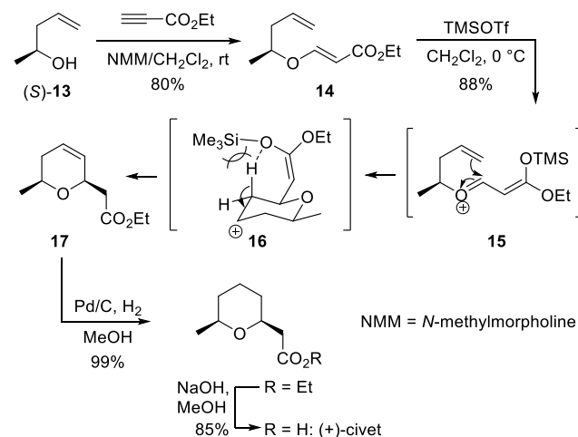
Scheme 9. Asymmetric synthesis of (+)-civet by \beta -alkoxyacrylate cyclisation.
