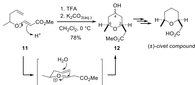
Scheme 8. Enol ether Prins -cyclisation in the total synthesis of (±)-civet.
