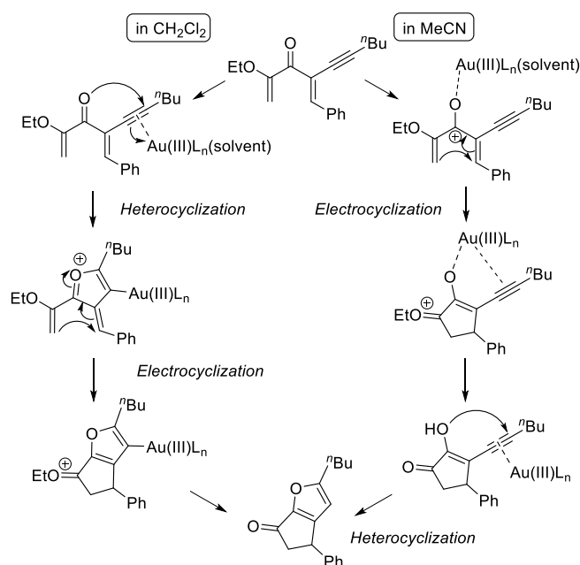
Scheme 37. Solvent-dependent mechanistic divergence in the gold-catalysed tandem heterocyclisation/Nazarov cyclisation of \alpha -ethoxy divinyl ketones.
