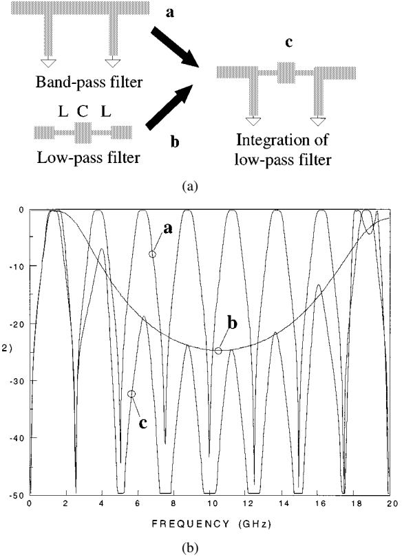
Fig. 3. Illustration of the low-pass filter insertion. (a) Integration of semilumped low-pass filter within the inverter of the bandpass filter. (b) Theoretical associated responses.
