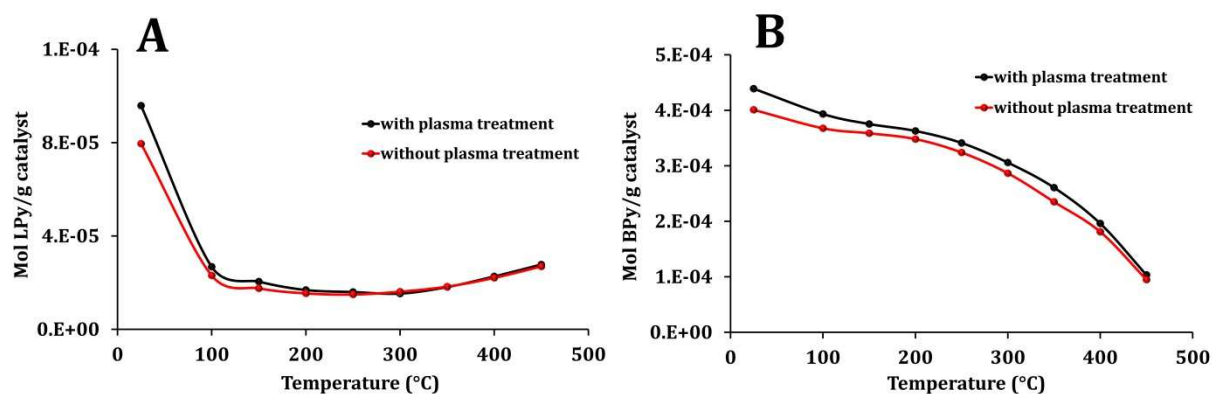
Figure 4: Number of moles of pyridine adsorbed onto Lewis (A) and Brønsted (B) acid sites acidity as a function of evacuation temperature. At 25\text{ }^{\circ}\text{C} , this number directly reflects the number of acid sites.
