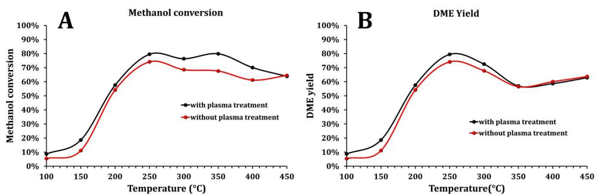
Figure 5: Catalytic activity of H-ZSM-5 zeolites with and without plasma activation
