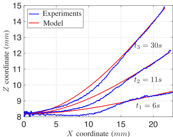
FIGURE 5. Experimental and modeled shapes of the polymer for different time values. The actuator is actuated at 2.5 V. Its length L is 24 mm.
