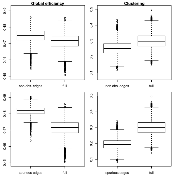
Figure 1: Influence of missidentifications of edges on Global Efficiency and on Clustering coefficient. 10000 simulations were done on 51 nodes small-world graphs with 153 edges. Missidentifications consist in 33% of spurious edges or 75% of only correctly observed edges, that is, in each case 51 edges misspecified.
