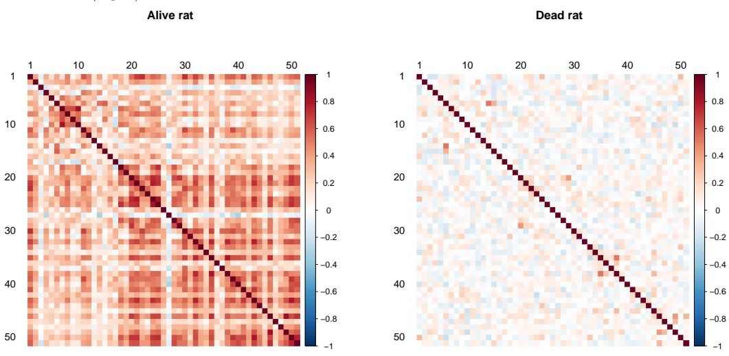
Figure 7: Examples of two correlation matrices between wavelet coefficients obtained at scale 4 for an alive rat (left) and a dead rat (right).
