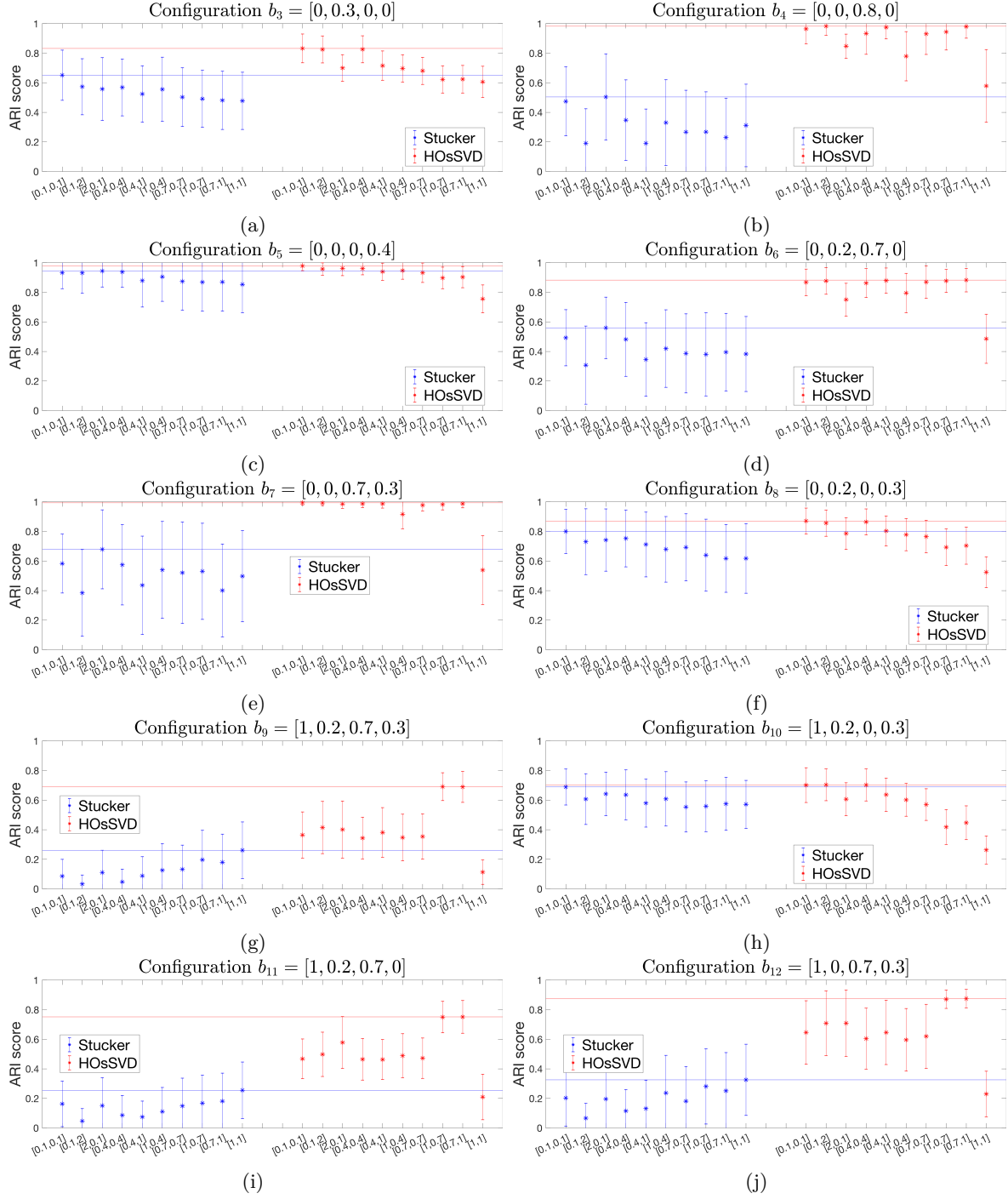
Figure 8: ARI score using SN-Tucker and HOsSVD algorithm in function of the sparsity parameters and the configurations
