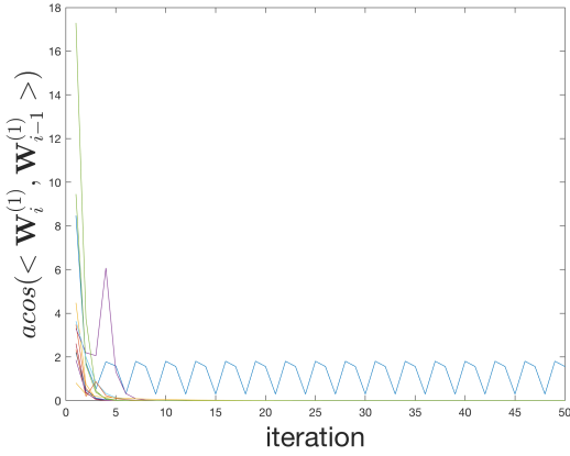
Figure 6: Convergence criteria for 12 realisation the experiment configuration b_{10} and [\gamma_1, \gamma_2] = [1, 1] .
