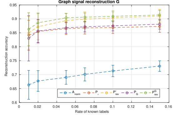
Fig. 4. Reconstruction of the graph signal f_0 on \mathcal{G} .
