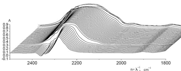
Figure 11 Infrared analyses at 22°C of the polyurethane system AT-FPG.
