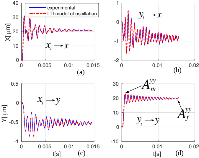
Fig. 11: Experimental characterization and model simulation of the step responses where the badly damped vibrations are illustrated.
