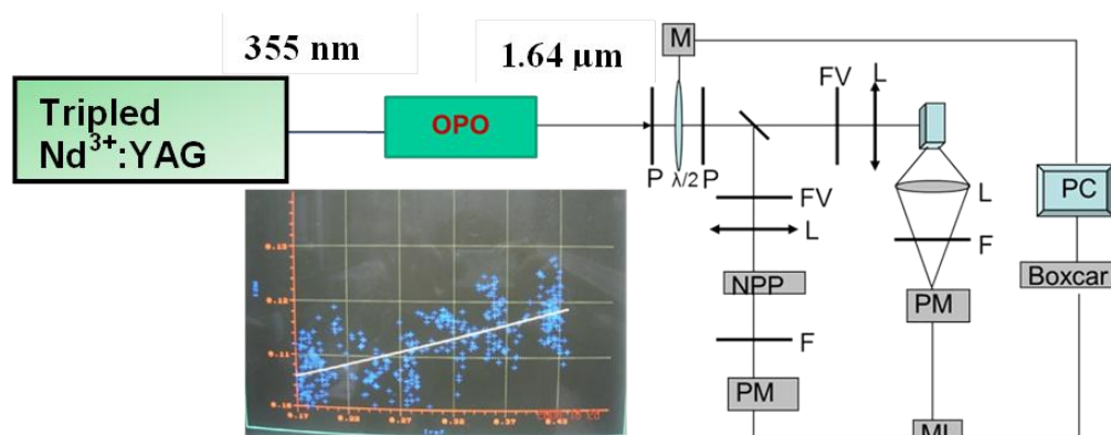
Figure 5. A schematic diagram of HRS measurement at 1.64 \mu\text{m} . F: Filter; M: Mirrors; A: Attenuator; GP: Glass plate; L: Lens; P: Polarizer; \lambda/2 : Half wave plate; PMT: Photomultiplier tube; NPP ( N -4-nitrophenyl-prolinol): Reference material.
