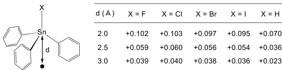
Figure 3. Electrostatic potential of \{(o\text{-H})\text{C}_6\text{H}_4\}_3\text{Sn(X)} (X = F, Cl, Br, I, H) at the position trans to the Sn–X bond.
