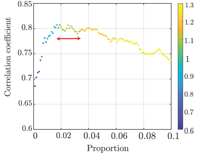
FIG. 9. Robustness of the inertia matrix method quality versus choice of parameter: correlation coefficient versus “proportion” parameter (see text), for the Drosophila pupa data set. The correlation slope is color coded. The method quality is optimal when the correlation coefficient is high and the slope close to 1. The red arrow represents the parameter range which can reasonably be used for this data set.
