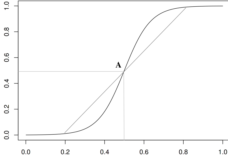
Figure 1: The logistic function. This function is often used to model a growth with constraints leading to a saturation. However, this function possess a center of symmetry, A , which implies that the initial exponential growth is exactly equivalent to the way the growth saturates. This is
