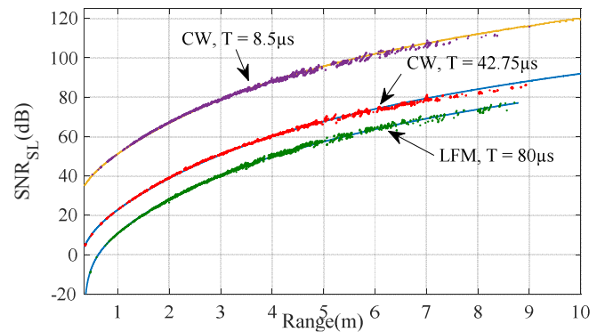
Figure 12 Baseline decorrelation effect; SNR to Horizontal Range
