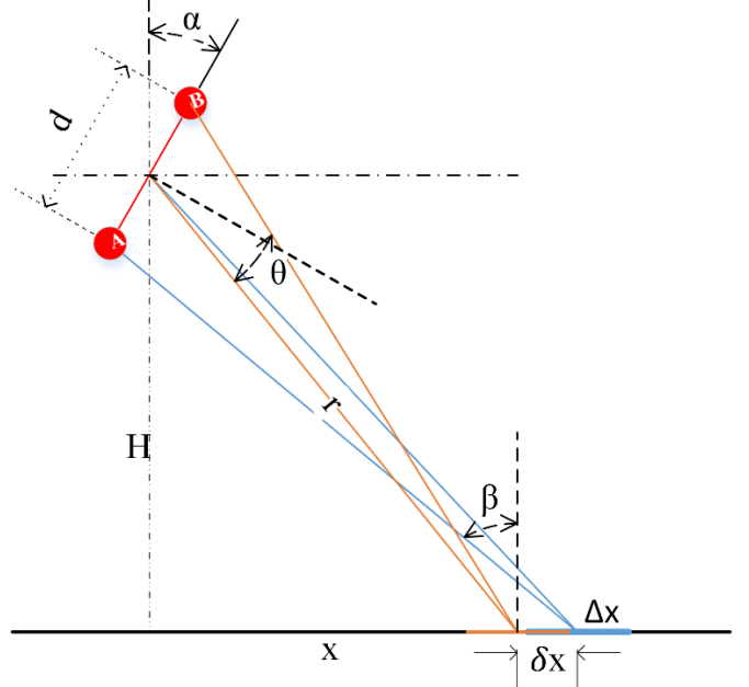
Figure 9 Sliding footprint effect demonstration, where \Delta x is footprint size and \delta x is shift in the footprint.
