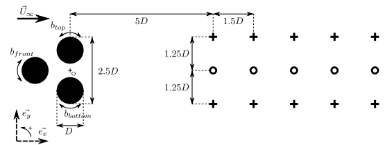
Fig. 1: Fluidic pinball configuration. b_{front} , b_{bottom} and b_{top} denote the peripheral speed of the cylinders. Circles downstream stand for y-velocity sensors and crosses x-velocity sensors. Axis origin is halfway between the two back cylinders.
