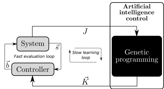
Fig. 2: Artificial intelligence control paradigm. A large number of evaluations of different control laws \vec{K} are performed to assess their performance J ( fast evaluation loop ), then genetic programming create new control laws based on the most performing ones ( slow learning loop )
