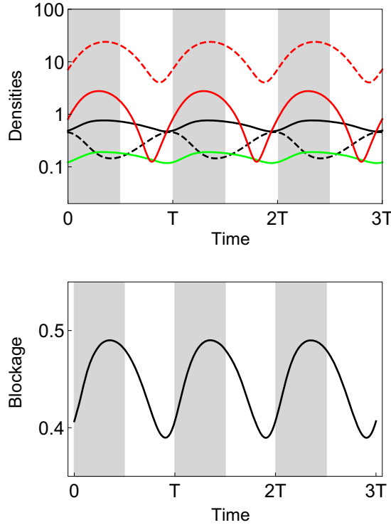
Figure 4. Epidemiology and evolution of plague in a seasonal environment. We allow the growth rate of the flea population \lambda_F(t) = 1 + \sin(2\pi t/T) to vary periodically ( T = 200 ) because of seasonality (the shaded area indicates time when the growth rate is above average, that is, when \lambda_F(t) > 1 ). We assume that two bacterial strains are competing but we do not allow for superinfection: one strain never blocks the flea ( \epsilon_1 = 0 ) and another strain can block infected fleas ( \epsilon_2 = 1 ). The two strains coexist, although blockage is maladaptive according to condition (5) in the absence of superinfection (i.e., \frac{\beta_B}{m_F + \alpha_B} \approx 0.119 < \frac{\beta_U}{m_F + \alpha_U} = 0.125 ) but their relative frequency fluctuates in synchrony with the incidence of the disease in the vector. Other parameter values (see Materials and Methods section for more details about the simulation procedure): \lambda_H = 0.01 , \gamma = 0.2 , \theta = 0.5 , \sigma = 0.3 , \delta = 2 , m_H = 0.004 , m_F = 0.02 , \alpha_H = 0.01 , \alpha_U = 0.02 , \alpha_B = 0.3 , \beta_H = 0.001 , \beta_P = 0.01 , \beta_U = 0.005 , \beta_B = 0.038 .
